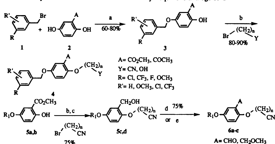
Scheme I Synthetic route for the 2-substituted hydroquinone analogs of I
