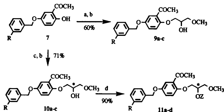
Scheme II Synthetic route to racemic and chiral secondary alcohols
